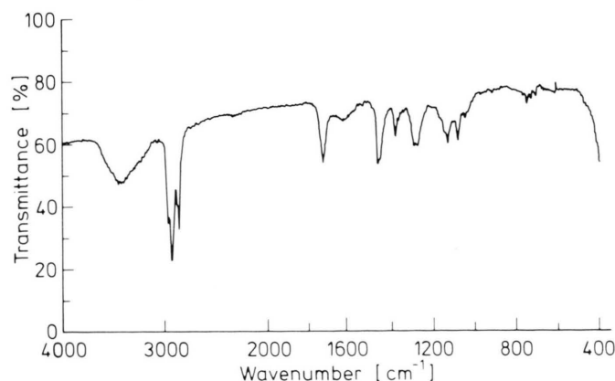
Fig. 1. IR spectrum of the total phosphonolipids isolated from beef brain right lobe.
